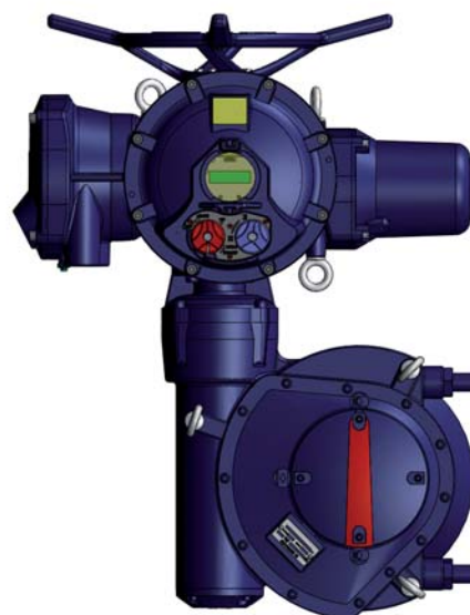
BERNARD CONTROLS STX actuator on a worm gearbox
